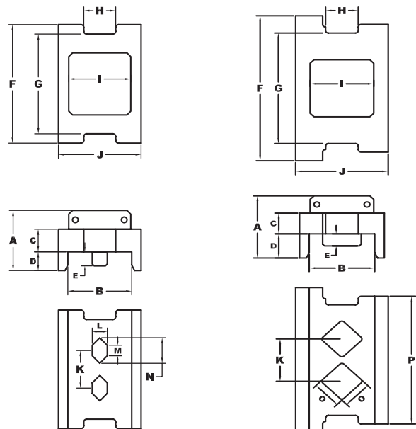
SHEET PILE INSERT DCS-1
